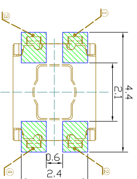
P.C.B MOUNTING PATTERN DIMENSION
